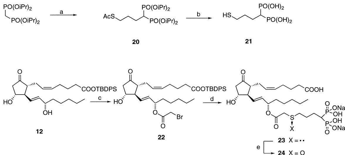
Scheme 5. Reagents: (a) \text{NaH} , \text{DMF} , \text{AcS}(\text{CH}_2)_3\text{I} (19); (b) \text{HCl} , reflux; (c) \text{BrCH}_2\text{COBr} , \text{THF} , \text{pyr} , -25^\circ\text{C} ; (d) 1) 21, \text{Et}_3\text{N} , dioxane, water. 2) DOWEX ( \text{Na}^+ ); (e) \text{CH}_3\text{COOOH} .
