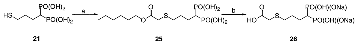
Scheme 6. Reagents: (a) \text{BrCH}_2\text{COOC}_6\text{H}_{13} , \text{EtN}(\text{iPr})_2 , dioxane; (b) 1) \text{HCl} , reflux. 2) \text{NaOH} .
