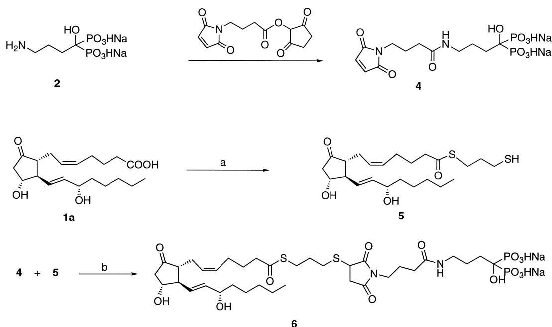
Scheme 2. Reagents: (a) HS(CH 2 ) 3 SH, DCC; (b) MeOH, H 2 O.
